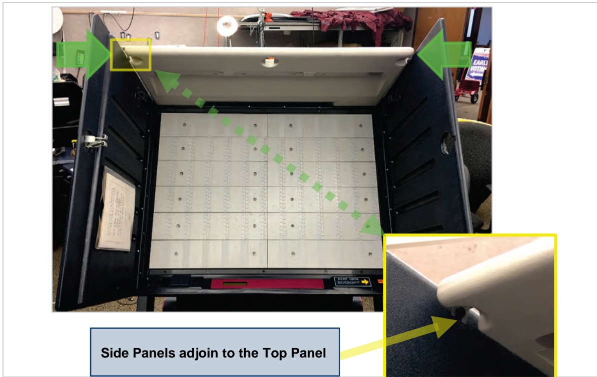
Figure 22: Connect the Top Panel with Side Panels
