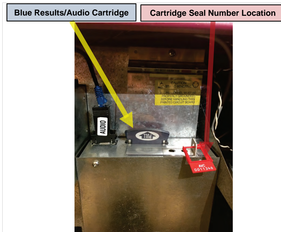
Figure 50: Results/Audio Cartridge Port Location and Removal (Part 1)
